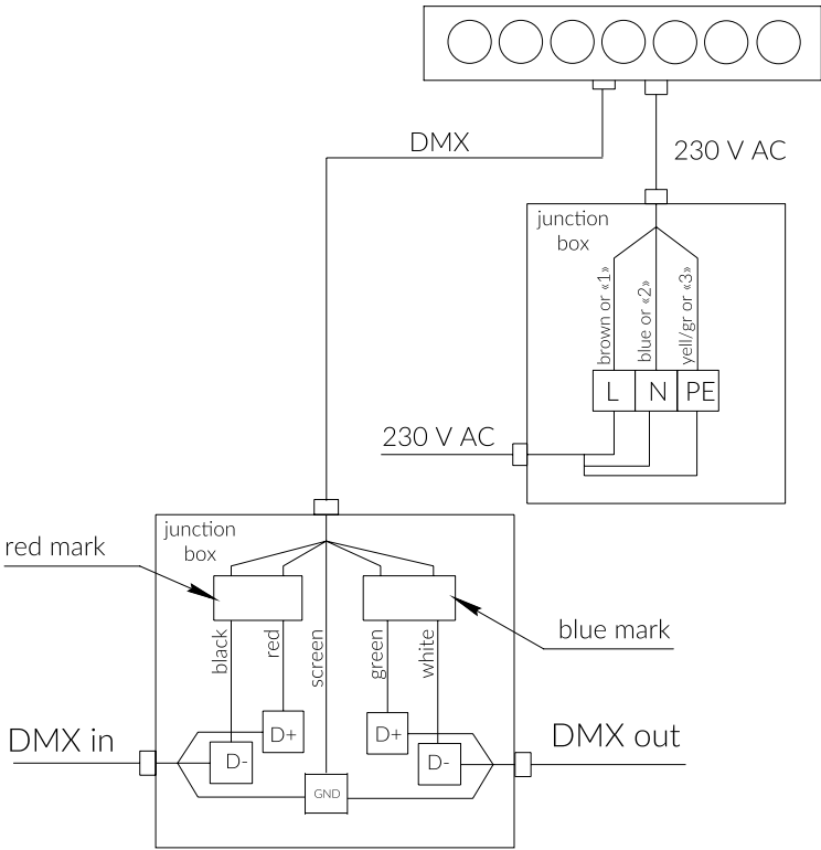
IntiLINE dynamic color luminaire connection diagram
