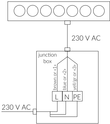
IntiLINE white color luminaire connection diagram
